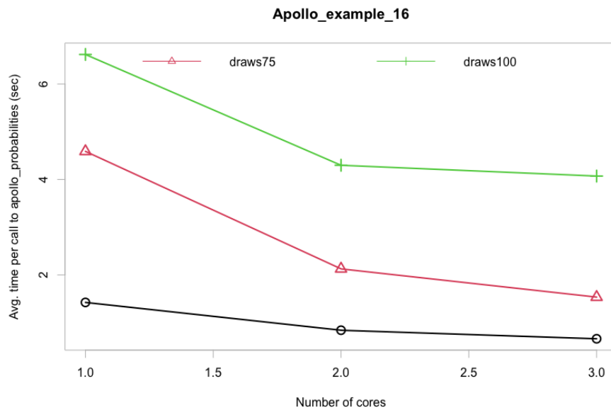
Figure 6.11: Running apollo_speedTest
