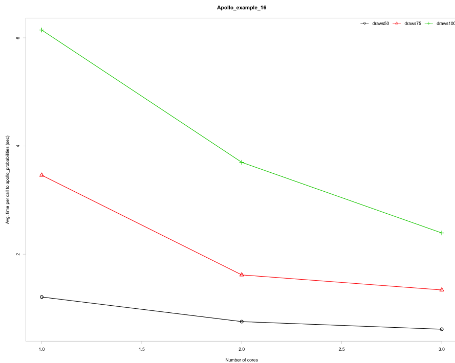
Figure 6.11: Running apollo_speedTest
